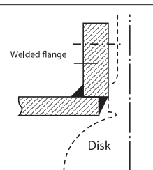
Double welding
